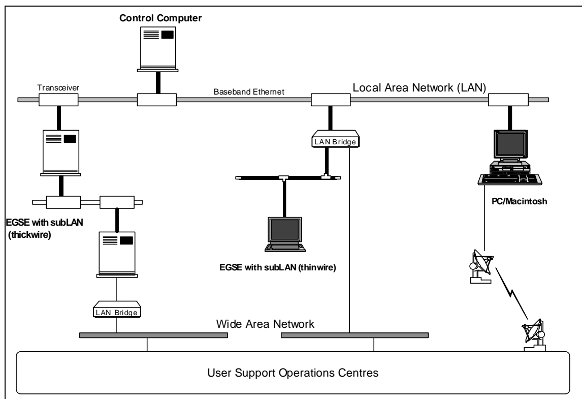
Figure 4 Overview of EGSE Connections to the EGSE LAN
