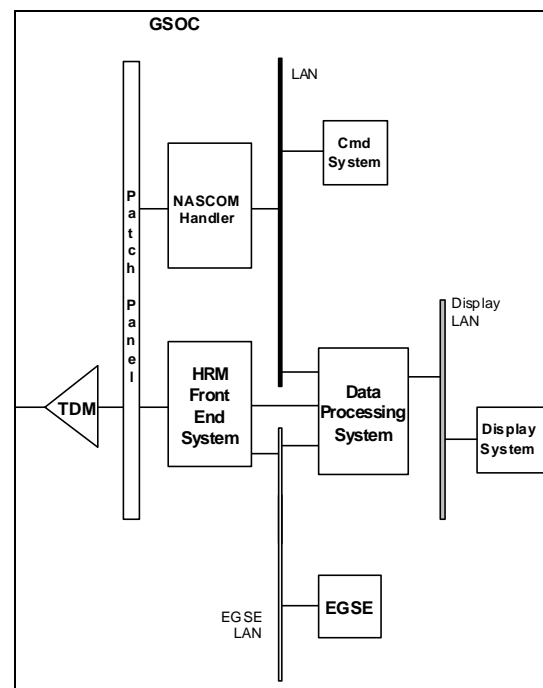
Figure 2 GSOC Functional Block Diagram
